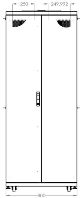
REAR VIEW
