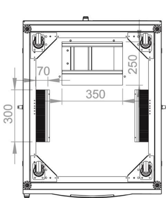
Bottom view
