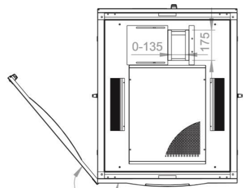
0°-230° Front door opening angle
