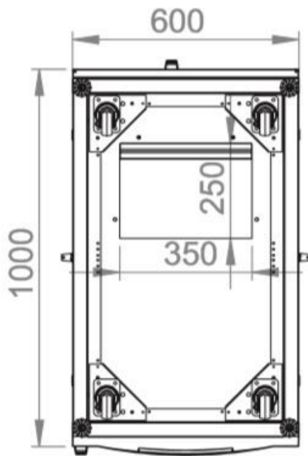
Bottom view
