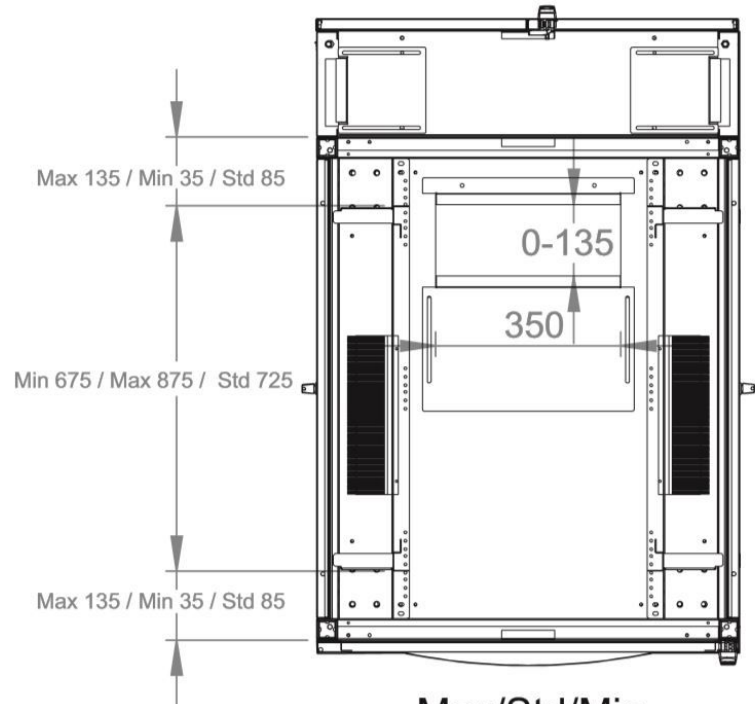
Max/Std/Min Equipment mounting Distance
