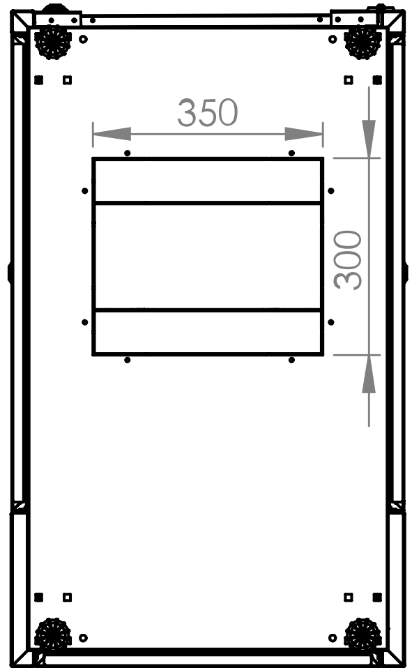
Bottom view
