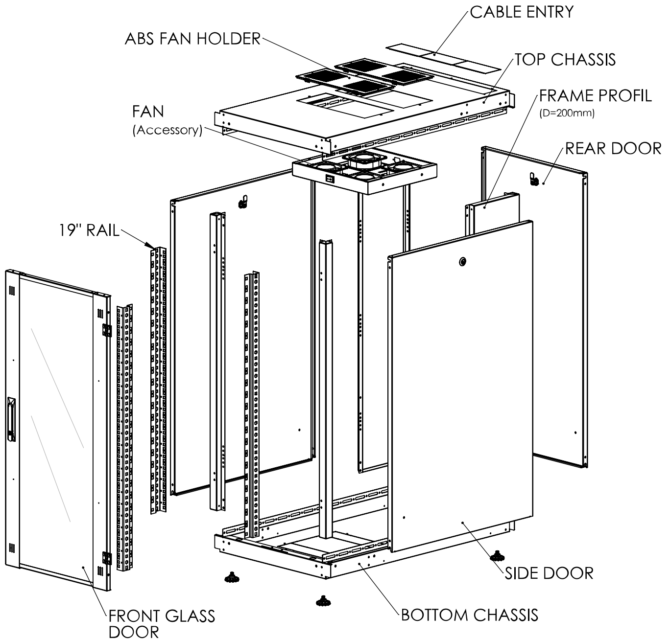
Exploded view
